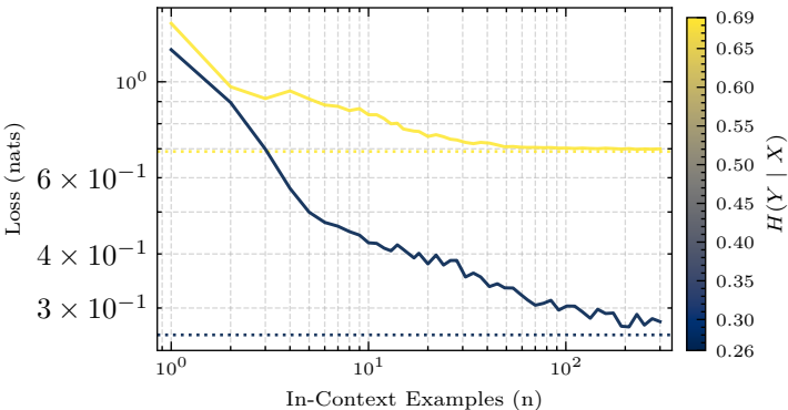
In-Context Learning Loss for Qwen-2.5 (32B)
